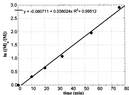
Figure 1. Plot of \ln([M]_0/[M]) vs time for ATRP of tBA at 60 °C in 20% p -dimethoxybenzene (DMB) with 5% added CuBr 2 : [tBA]_0 = 5.6 M; [\text{methyl 2-bromopropionate}]_0 = 0.11 M; [CuBr_2]_0 = 56 mM; [PMDETA]_0 = 58 mM; [CuBr_2]_0 = 2.8 mM.
