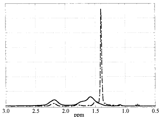
Figure 10. ^1H NMR spectra of p(tBA) ( M_n = 5300 , M_w/M_n = 1.33 ) before (dotted line, CDCl_3 ) and after hydrolysis (solid line, D_2O ). Both spectra were recorded at room temperature.
