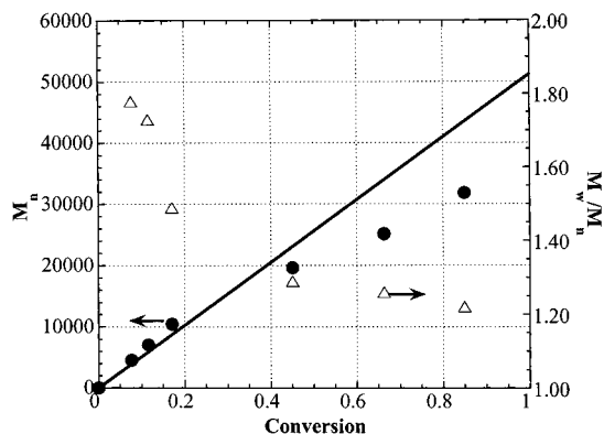
Figure 7. Plot of M_n and M_w/M_n vs conversion for ATRP of tBA at 70 °C in bulk: [tBA]_0 = 6.8 M; [methyl\ 2-bromopropionate]_0 = 16 mM; [CuBr]_0 = 16 mM; [PMDETA]_0 = 16 mM.
