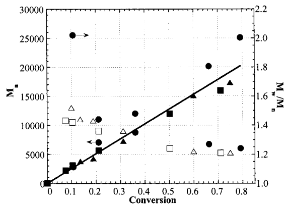
Figure 9. Plot of M_n (closed symbols) and M_w/M_n (open symbols) vs conversion for ATRP of tBA at 70 °C in bulk: [tBA]_0 = 6.8 M; [dimethyl\ 2,6-dibromoheptanedioate]_0 = 34 mM; [CuBr]_0 = 17 mM; [PMDETA]_0 = 17 mM; (●, ○×b0) not separate solutions, (▲, △×90) separate initiator and catalyst solutions, (■, □) separate initiator and catalyst solutions with a vigorous deoxygenation of the initiator solutions.
