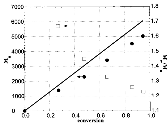
Figure 2. Plot of M_n and M_w/M_n vs conversion for ATRP of tBA at 60 °C in 20% p -dimethoxybenzene (DMB) with 5% added CuBr 2 : [tBA]_0 = 5.6 M; [\text{methyl 2-bromopropionate}]_0 = 0.11 M; [CuBr_2]_0 = 56 mM; [PMDETA]_0 = 58 mM; [CuBr_2]_0 = 2.8 mM.
